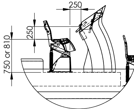
DETAIL A SCALE 1 : 50
